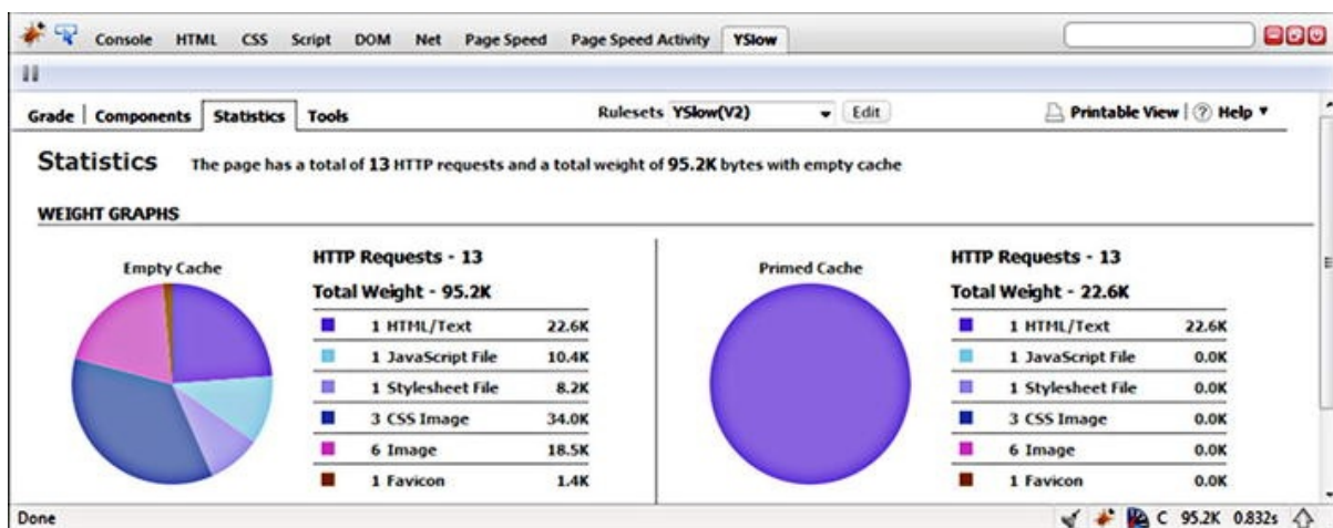
YSlow statistics tab
